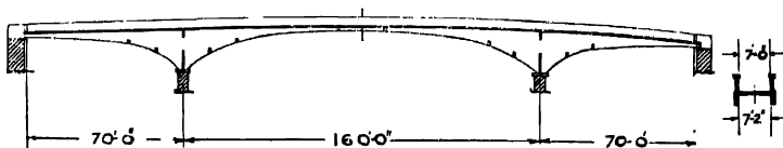
Fig. 347.—Footbridge over River Forth, Stirling.
